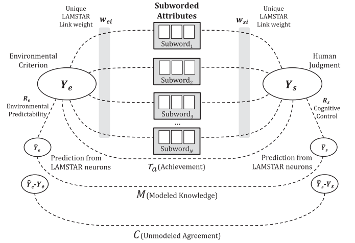
Fig. 4. Graphical representation of LAMSTAR-based JA. Note that i is an integer with range [1, N] .
