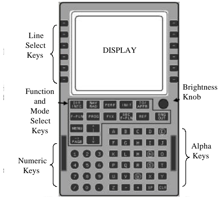
Figure 4. MCDU Layout
