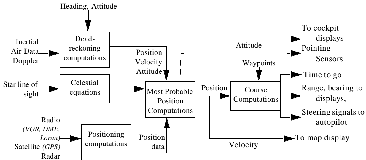
Figure 3. Navigation System [14]
