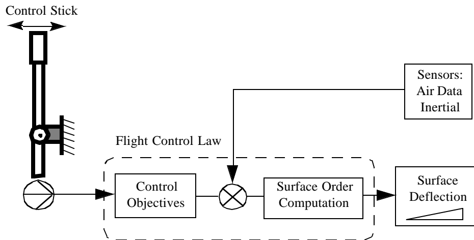
Figure 5. Flight Control System Architecture
