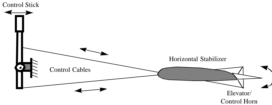
Figure 1. Mechanical Flight Control System
