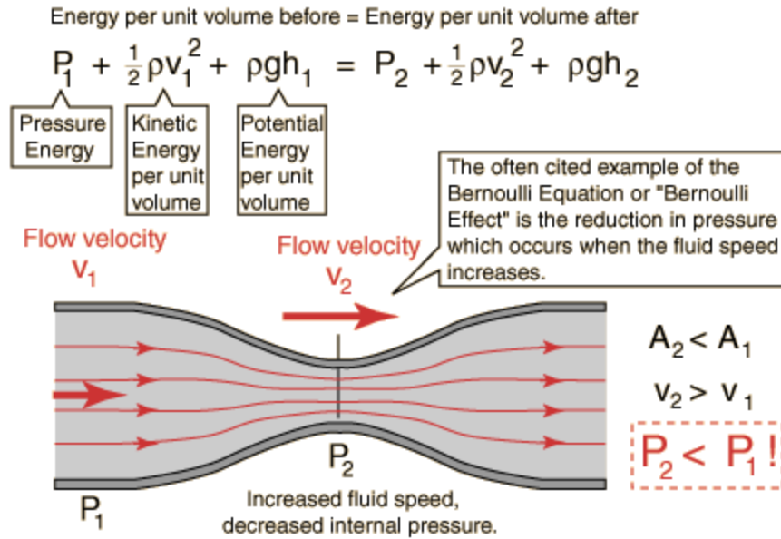
Figure 2. Depiction of the Bernoulli effect[1]
