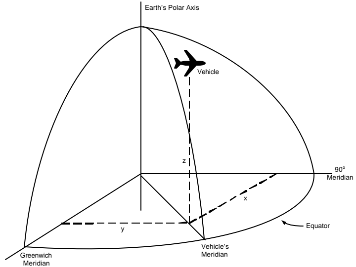
Figure 1. x, y, z Coordinate Frame[13]
