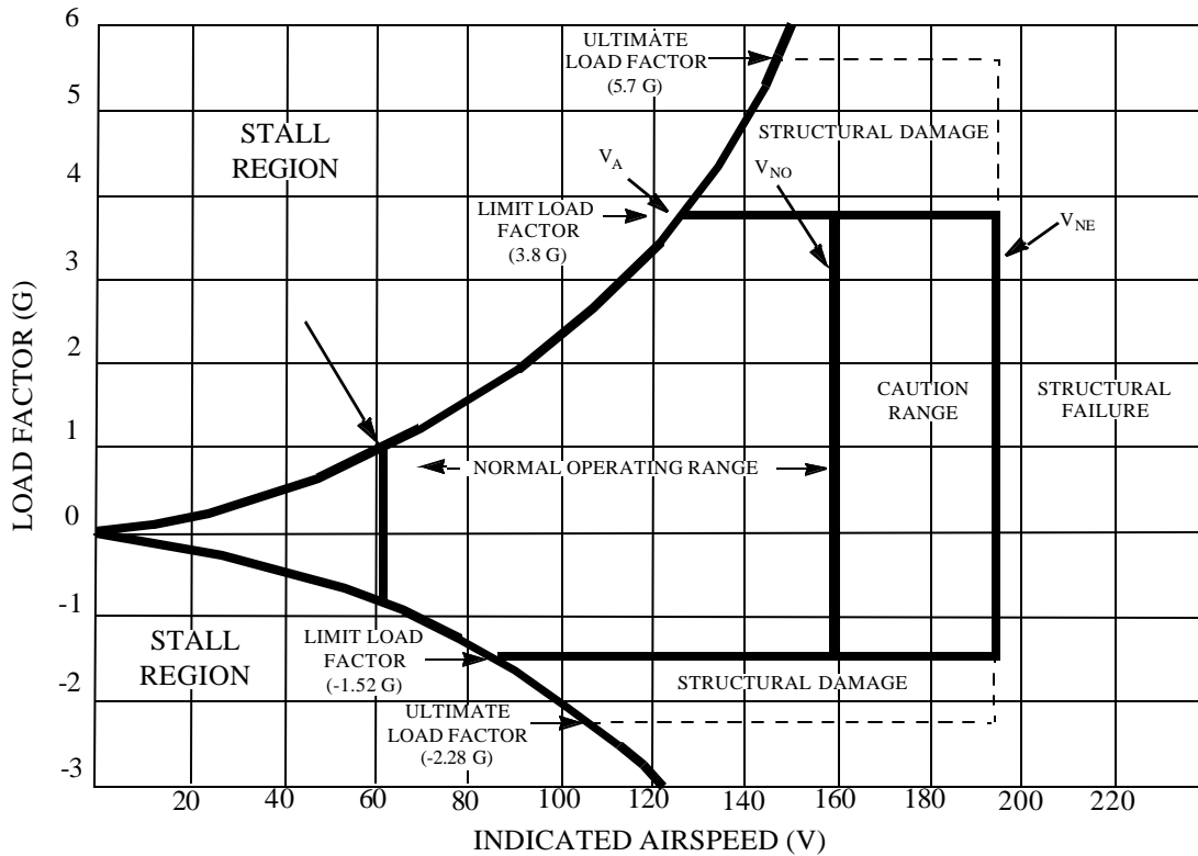
Figure 4. Typical Flight Envelope[6]
