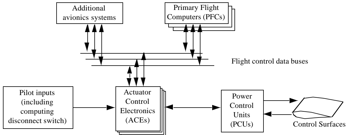
Figure 6. Boeing 777 Primary FCS Overview (excerpted from Yeh [13])
