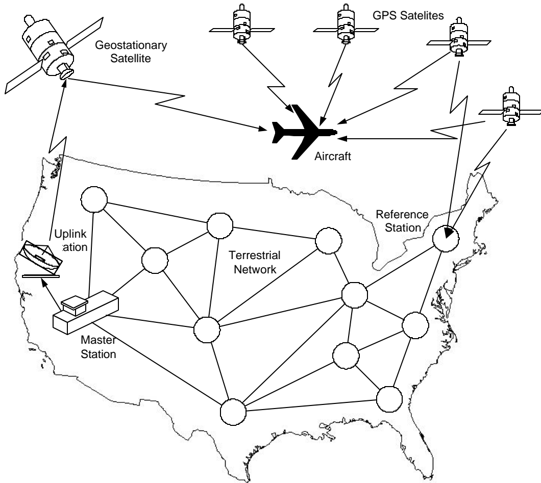
Figure 2. The Wide Area Augmentation System (WAAS)
