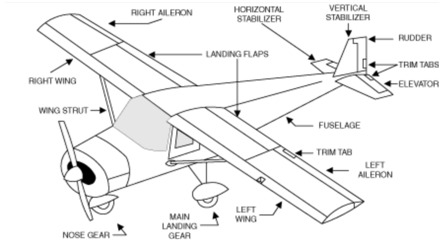
Figure 10. Aircraft Control Surfaces[6]
