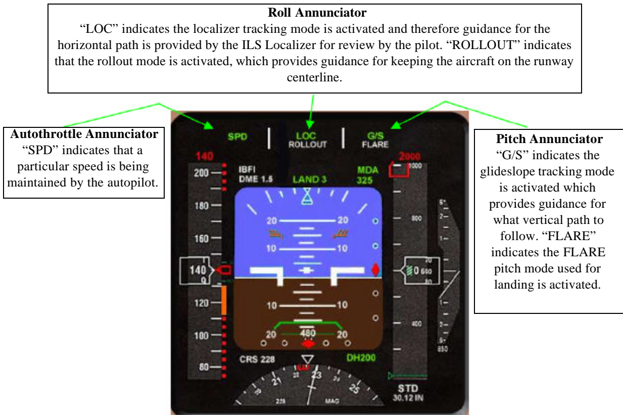
Figure 2. MD-11 (top) and B-747 [14] (bottom) Primary Flight Displays
