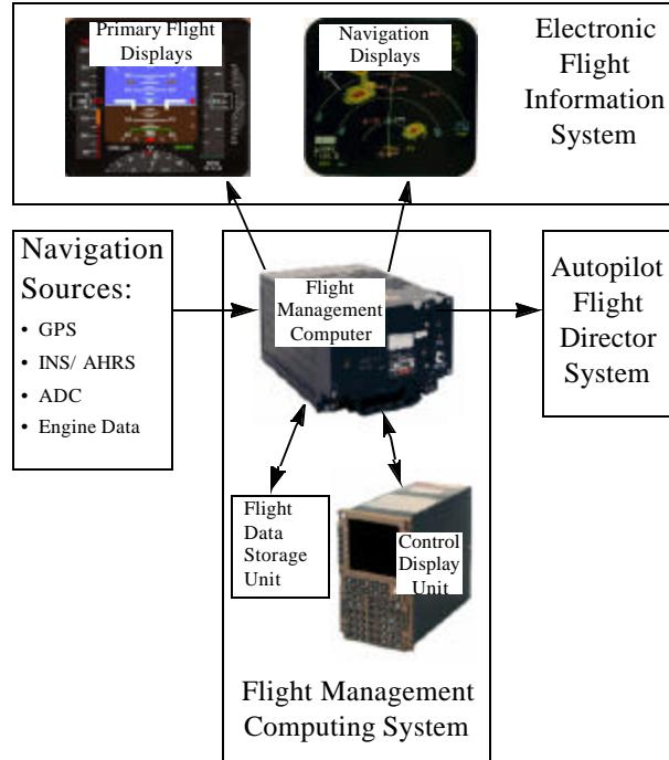
Figure 7. FMS Components
