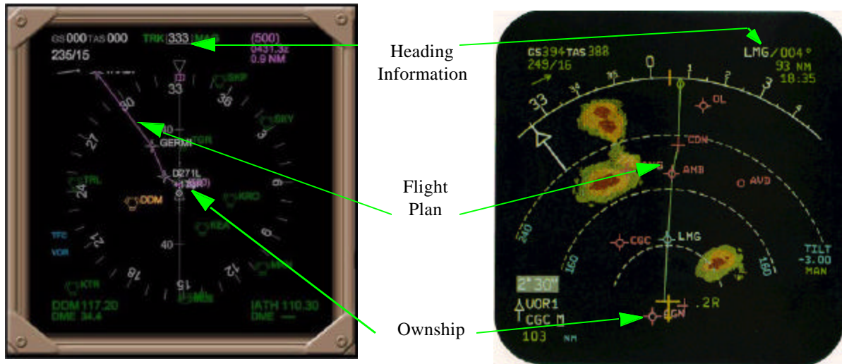
Figure 6. Boeing 777 ND [14] (left) and A320 ND [5] (right)
