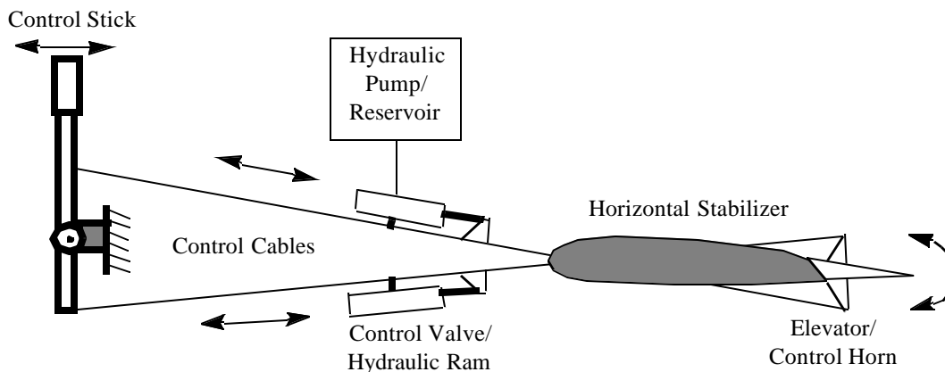
Figure 2. Boosted Flight Control System
