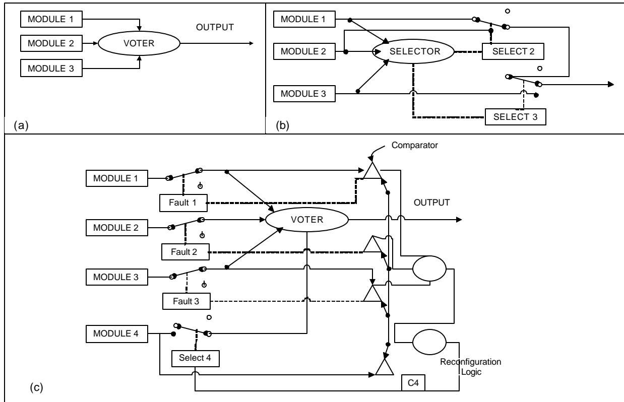
Figure 1. Basic Forms of Redundancy
