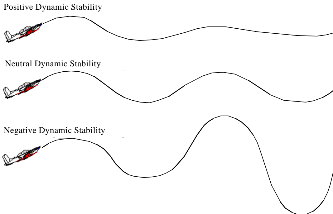
Figure 9. Positive, Neutral, and Negative Dynamic Stability [5]
