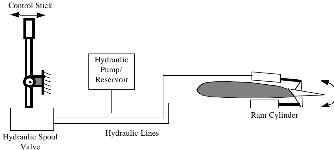
Figure 3. Hydraulic Flight Control System
